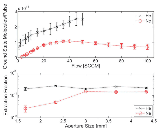
Fig. 12 Top: Number of absolute ground state molecules output per pulse with helium and neon buffer gases, using a 4.5 mm cell aperture. Bottom: Fraction of molecules extracted out of the cell into the beam, with neon and helium buffer gases.
