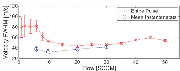
Fig. 11 The velocity spread in the forward direction with helium buffer gas. The data points marked by the \times symbols indicate velocity spread averaged over the entire molecule pulse, while the data points marked by the \circ symbols indicate the mean instantaneous velocity spread obtained from time-resolved fluorescence data.
