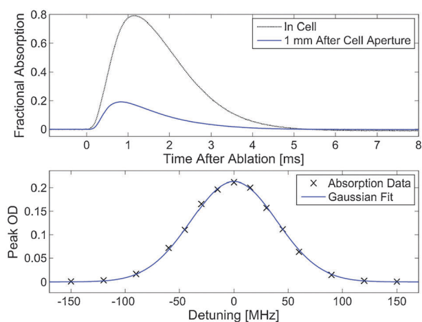
Fig. 2 Top: An absorption signal of the ThO molecular beam in a 1 SCCM flow of helium buffer gas with a 4.5 mm diameter cell aperture. The laser is fixed spatially, so the time variation of the signal is a result of the molecular beam pulse passing through the laser. The different traces show absorption in the cell (dotted) and 1 mm after the cell aperture (solid). For these data, the laser is locked on the resonance of the X-C Q(1) line. The width and height of the signals depend on the buffer gas flow rate, buffer gas species, and cell aperture size; however, the qualitative features are similar. Bottom: By varying the laser detuning, we obtain an absorption spectrum. This curve shows the absorption spectrum of the molecular beam 1 mm after the cell, with the same experimental parameters as in the top figure. Optical density (OD) is defined as T = e^{-\text{OD}} , where T is the transmitted fraction of the probe laser light.
