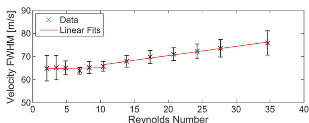
Fig. 9 The transverse spectral width vs. Reynolds number with neon buffer gas and a 4.5 mm cell aperture, measured at the aperture. At low flows the transverse widths inside the cell and outside the cell are the same, and indicate a thermal distribution of T \approx 20 K. The slope of the fit line at these low flows is (0.06 \pm 0.27) \text{ m s}^{-1} , consistent with zero. At higher flows the transverse width in the beam begins to linearly increase, with slope (0.41 \pm 0.06) \text{ m s}^{-1} . Note that the transition Reynolds number agrees with that from Fig. 7. For this aperture size, the conversion from flow to Reynolds number is Re \approx 0.7 \times \text{flow}/(1 \text{ SCCM}) .
