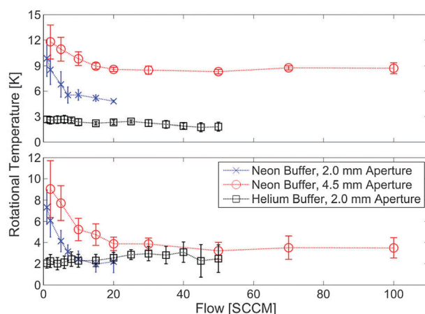
Fig. 3 Rotational temperatures in the buffer gas cooled beam. Top: Temperatures measured 1 mm from the cell aperture. Bottom: Final rotational temperatures in the expansion, measured 6 cm after the cell aperture. The cell temperatures are 5 \pm 1 \text{ K} and 18 \pm 1 \text{ K} for helium and neon buffer gases, respectively. The data with a helium buffer gas were taken with a 2.0 mm aperture, while the data with a neon buffer gas were taken with both 2.0 mm and 6.5 mm apertures.
