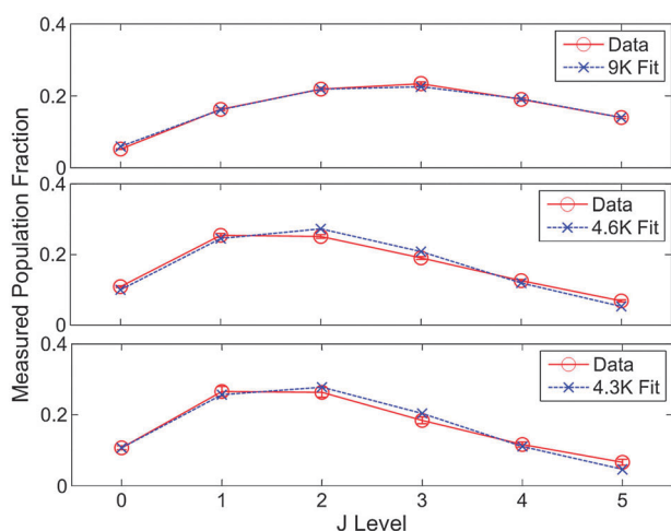
Fig. 4 Rotational level populations with Boltzmann distribution fits for 30 SCCM neon flow, 4.5 mm aperture. The top, middle, and bottom plots show the distributions 1 mm, 2 cm, and 6 cm from the cell aperture, respectively.
