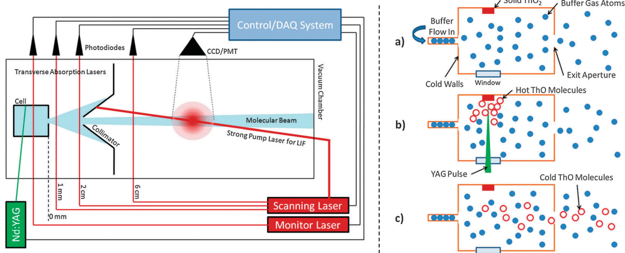
Fig. 1 Left: The cold beam apparatus. The features inside the vacuum chamber are described in Section 2, and the features outside the vacuum chamber are described in Section 3. Right: A detailed view of the cell. (a) A continuous gas flow maintains a stagnation density of buffer gas atoms (filled blue circles) in thermal equilibrium with a cold cell. A solid piece of ThO 2 is mounted to the cell wall. (b) A YAG pulse vaporizes a portion of the target and ejects hot ThO molecules (empty red circles). (c) Collisions with the buffer gas cool the molecules, which then flow out of the cell to form a beam.
