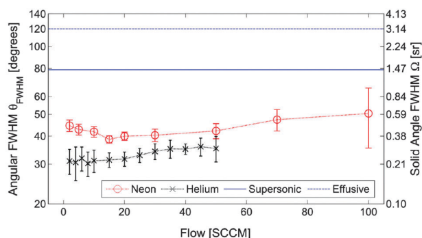
Fig. 8 Divergence in the beam with a 4.5 mm aperture, measured 2 cm after the cell aperture, compared to the divergences of supersonic and effusive beams. 2 The cell temperatures are 18 \pm 1 K for neon, 5 \pm 1 K for helium. For this aperture size, the conversion from flow to Reynolds number is Re \approx 0.7 \times \text{flow}/(1 \text{ SCCM}) .
