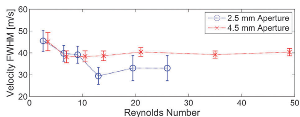
Fig. 10 The velocity spread in the forward direction with neon buffer gas.
