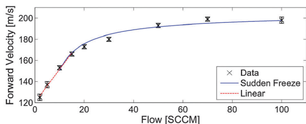
Fig. 7 Forward velocity for neon buffer gas with a 4.5 mm aperture, along with a linear fit at low flow and a sudden freeze fit at high flow. The sudden freeze fit is to the function v = \alpha\sqrt{1 - \beta f^{-4/5}} , with parameters \alpha = 205 \pm 6 \text{ m s}^{-1} , \beta = 3.0 \pm 0.5 . The parameters are close to the expected values of \alpha \approx 200 \text{ m s}^{-1} (the final velocity) from experiment, and \beta \approx 3 from the estimate above. The linear model has a slope of 3.1 \pm 0.8 \text{ (m s}^{-1}) \text{ per SCCM} , in good agreement with our estimate of 4.5 \text{ (m s}^{-1}) \text{ per SCCM} .
