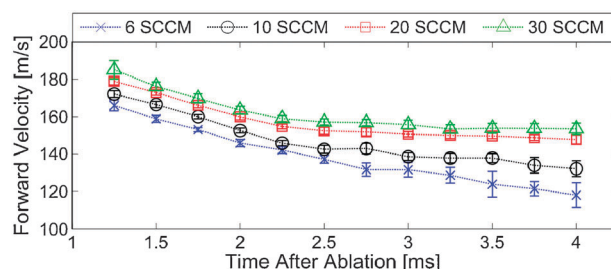
Fig. 6 Forward velocity vs. time after ablation for several different flow rates of the helium buffer gas.
