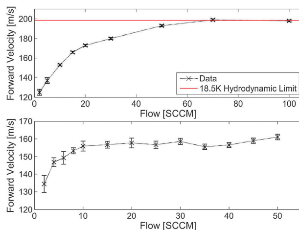
Fig. 5 Top: Mean forward velocity vs. flow rate with neon buffer gas. The solid line is the hydrodynamic limit for the forward velocity of neon atoms exiting an 18.5 K cell, given by eqn (4). The forward velocity of the molecules with neon buffer gas cooling varies by no more than 10% over a pulse. Bottom: Mean forward velocity vs. flow rate with helium buffer gas.
