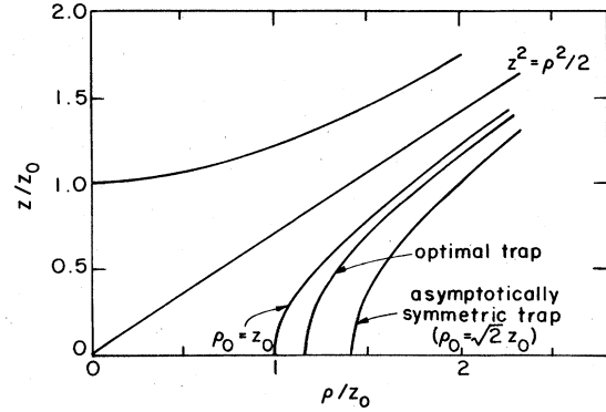
FIG. 49. Contours for the hyperbolic electrodes for a trap with \rho_0 = z_0 , an optimal trap, and an asymptotically symmetric trap. The endcap contour is shared by all three configurations.
