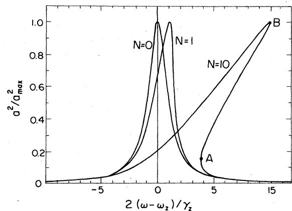
FIG. 11. Squared amplitude of an anharmonic oscillation vs the frequency of the driving force for three values of the anharmonicity parameter N defined by Eq. (3.79b). For N=0 the response curve is the familiar Lorentzian. For the critical value N=1 , the response is skewed to the right but remains single valued. With N > 1 the response has a triple-valued region, as illustrated by the curve for N=10 .
