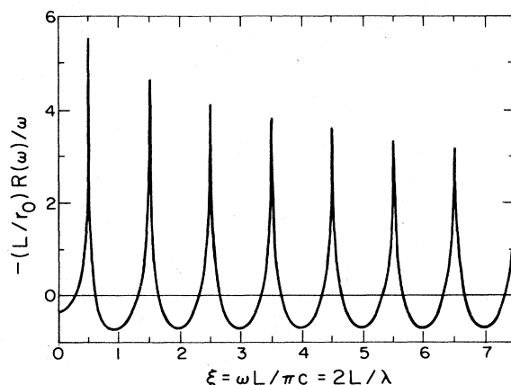
FIG. 37. Plot of the frequency shift -(L/\omega r_0)R_P(\omega) vs \xi for the cyclotron motion of a charged particle in the midplane between two imperfect conducting plates with \delta/L = 1 \times 10^{-3} .
