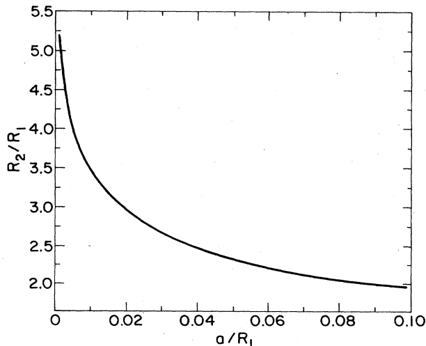
FIG. 31. "Magic" ratio R_2/R_1 for the two-loop scheme as a function of the scaled wire radius a/R_1 .
