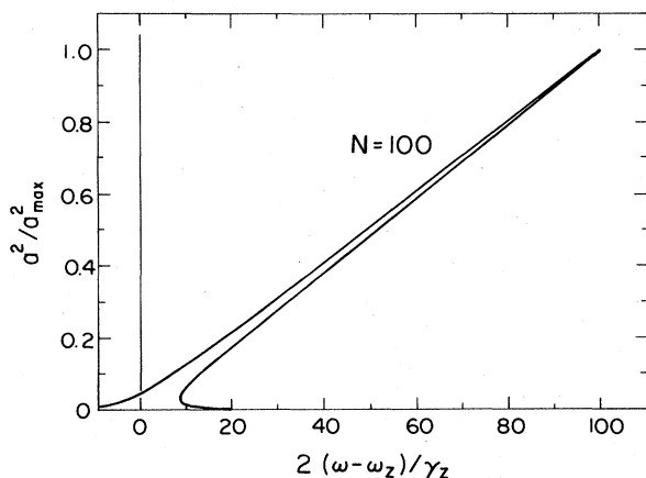
FIG. 14. Squared amplitude of an anharmonic oscillation vs the frequency of the driving force for a large value of the anharmonicity parameter, N = 100 .
