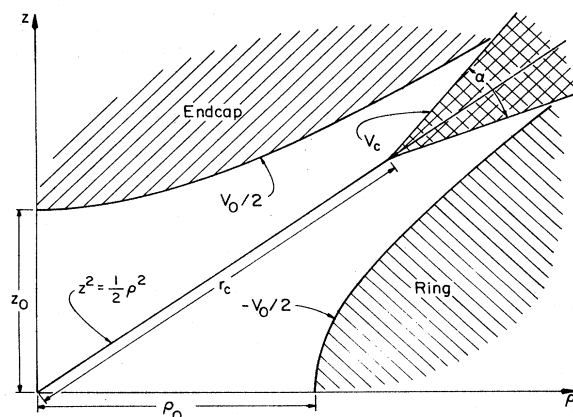
FIG. 43. Model of a hyperbolic Penning trap, which is invariant under rotations about the z axis and under the reflection z \rightarrow -z .
