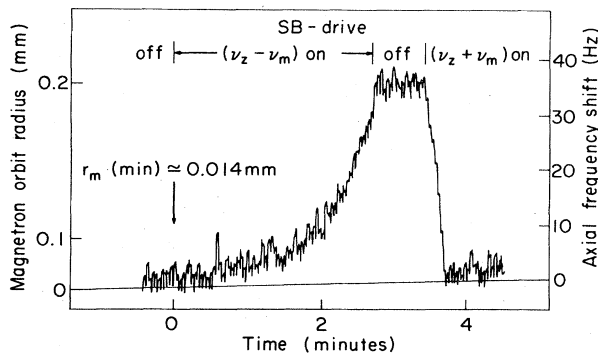
FIG. 17. Demonstration of sideband cooling and heating by Van Dyck, Schwinger, and Dehmelt (1978). Changes in the axial oscillation frequency (vertical scale) are proportional to the square of the magnetron radius because of the presence of a magnetic bottle and are monitored as a function of time (horizontal scale).
