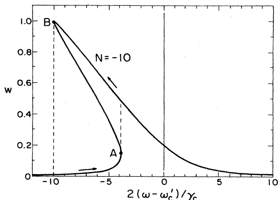
FIG. 32. Nonlinear, relativistic cyclotron resonance.
