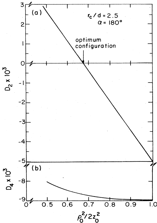
FIG. 48. Illustration of the different dependence of D_2 and D_4 upon the choice of hyperbolic surfaces represented by \rho^2/2z_0^2 . The optimal electrode configuration with \gamma = D_2 = 0 is indicated.
