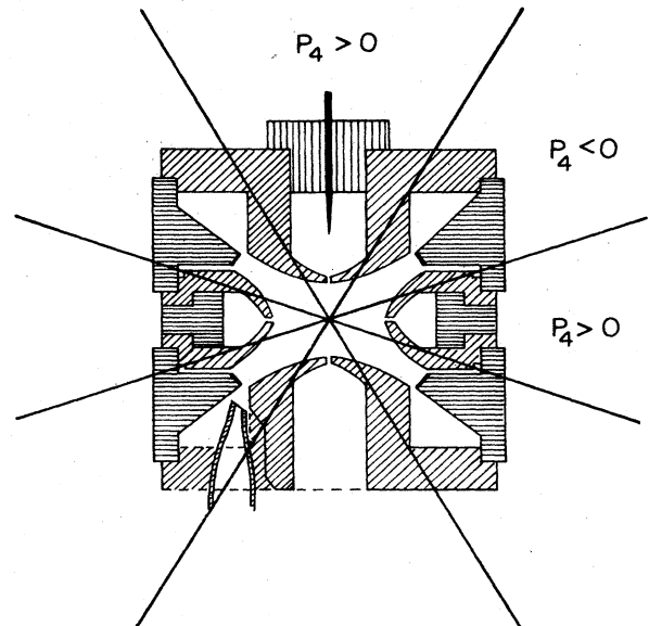
FIG. 25. The zeros of P_4(\cos\theta') superimposed over the Penning trap of Fig. 1.
