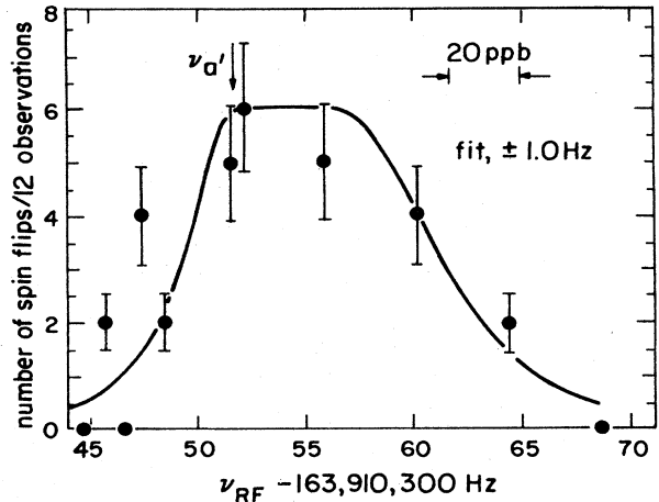
FIG. 29. Experimental anomaly resonance that is saturated. The solid curve is a fit to the line profile function (6.33), including the exponentiation given in Eq. (6.35). The g value determined from this fit and a simultaneous measurement of the cyclotron frequency is consistent with that deduced from the run shown in Fig. 28 (Van Dyck, Schwinger, and Dehmelt, 1984).
