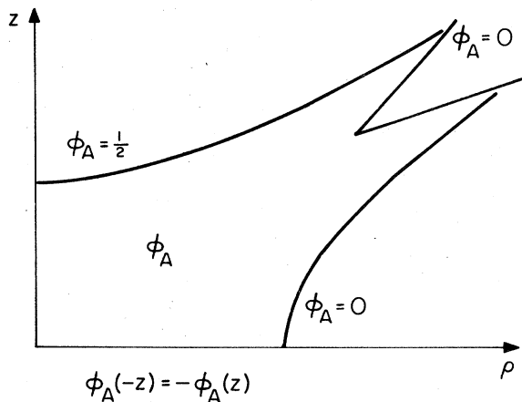
FIG. 51. Boundary conditions satisfied by \varphi_A . The boundary is invariant under rotations about the z axis and is antisymmetric under the reflection z \rightarrow -z .
