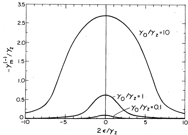
FIG. 20. Line shapes of the heating rate -\gamma_m^{(-)} , as given by Eq. (4.15) for several values of \gamma_0/\gamma_z . With appropriate interpretation, these line shapes apply to the analogous decay constants of Sec. III.C as well.
