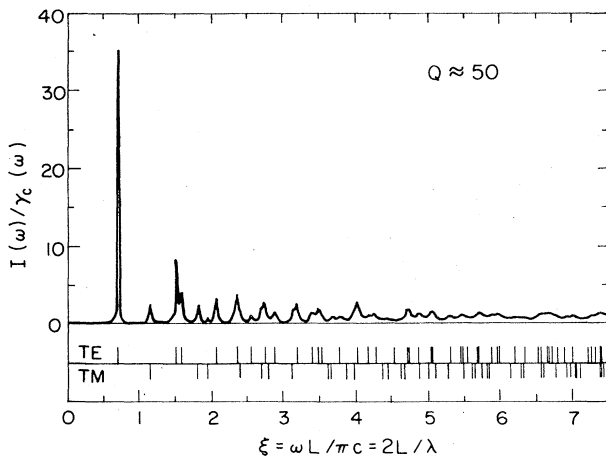
FIG. 38. The decay constant I(\omega)/\gamma_c(\omega) for a charged particle moving in a small orbit about the axis and centered in the midplane of a cylindrical cavity with Q = 50 and an aspect ratio R/L = 1.186 . The ticks denote the positions of the TE and TM modes.
