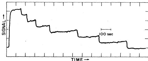
FIG. 5. Steps in the detected axial signal that appear when the axial drive is increased sufficiently to drive one electron at a time out of the trap. It is evident that there were initially seven electrons in the trap. The initial and final signal level is the noise floor (Wineland, Ekstrom, and Dehmelt, 1973).
