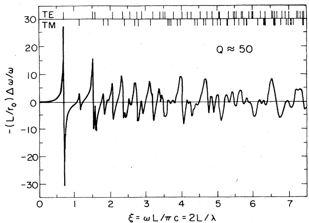
FIG. 39. Frequency shift corresponds to the decay constants of Fig. 38.
