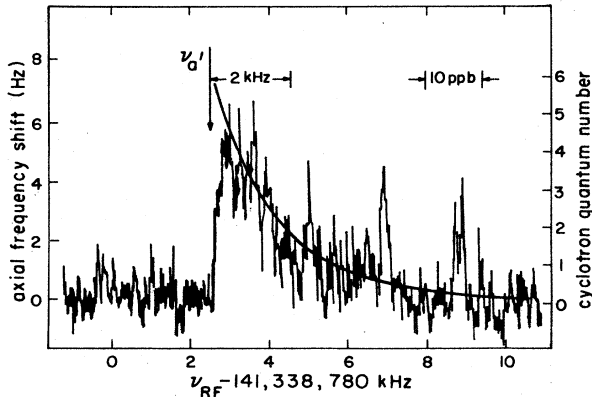
FIG. 27. Experimental cyclotron resonance. The solid curve is that given by Eq. (6.24) (Van Dyck, Schwinger, and Dehmelt, 1984).
