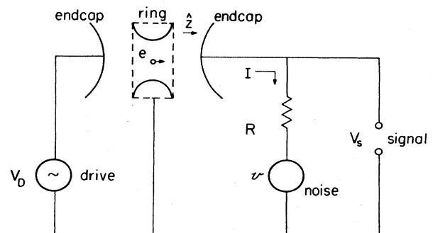
FIG. 9. Idealization of the radio-frequency circuit used to damp and detect the axial oscillation of a trapped particle. A charge e moving toward the right induces a current I through the resistor. The axial motion is driven by the oscillatory potential V_D and by the Johnson noise from the resistor v , while the signal voltage V_S is detected.
