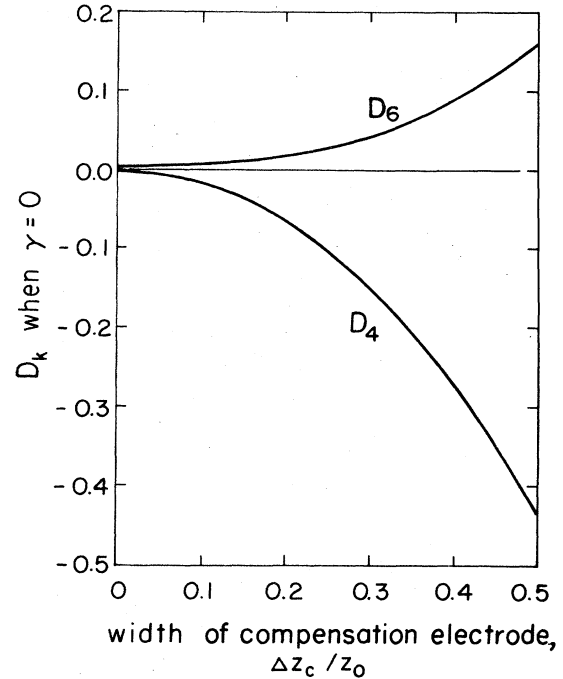
FIG. 59. The coefficients D_4 and D_6 as a function of the width of the compensation electrode, for a cylindrical trap with \rho_0/z_0 chosen to make \gamma=0 .
