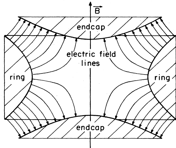
FIG. 2. Electric and magnetic field configurations of the Penning trap.
