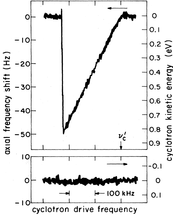
FIG. 33. Experimental observation of the relativistic cyclotron resonance (Gabrielse, Dehmelt, and Kells, 1985).
