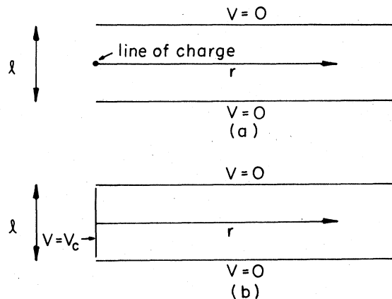
FIG. 46. Two-dimensional screening models. Parallel flat plate electrodes screen the potential produced (a) by a line of charge and (b) by a perpendicular electrode. In both cases, for r \gg l , a screening of the potentials by a factor of \exp(-\pi r/l) results.
