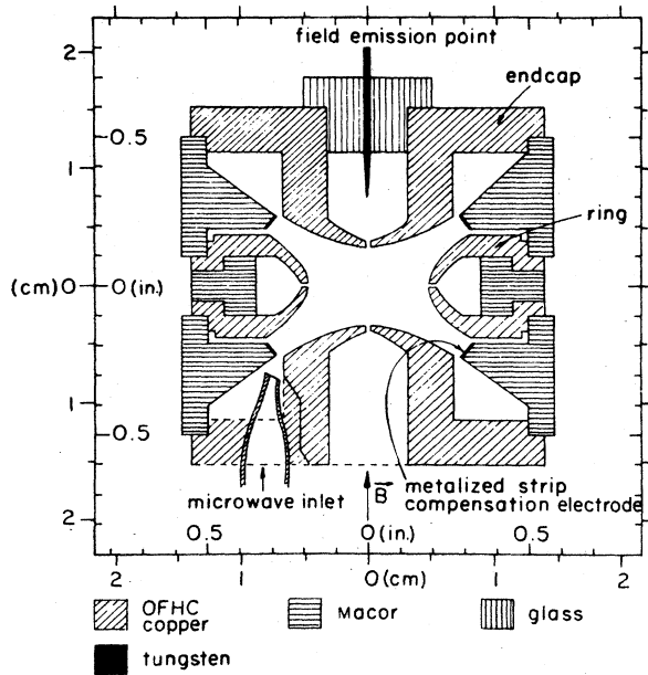
FIG. 1. Scale drawing of an experimental Penning trap (Gabrielse and Dehmelt, 1985).
