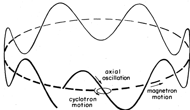
FIG. 3. Orbit of a charged particle in a Penning trap. The dashed line is the large and slow magnetron circle component of the motion. This, added to the axial oscillation, produces the guiding-center motion shown by the solid line. The total motion is given by adding the fast but small cyclotron circular motion about this moving guiding center. (Adapted from Ekstrom and Wineland, 1980.)
