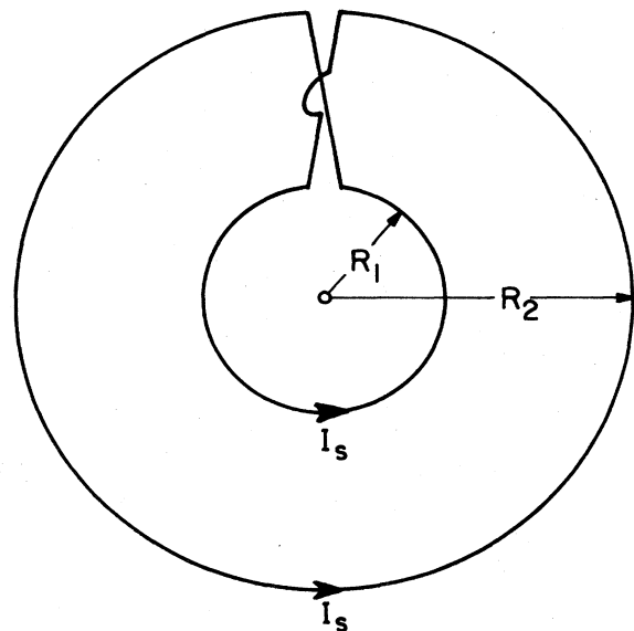
FIG. 30. Two-loop superconductor scheme of Van Dyck, Moore, Farnham, and Schwinberg (1986). With the "magic" ratio of R_2/R_1 (which depends on the wire radius a ), switching on a perpendicular uniform magnetic field does not change the value of the magnetic field at the center, but it does induce a bottle field. (We assume that the wires connecting the two loops are close together in comparison with their radius, so that their effects can be neglected.)
