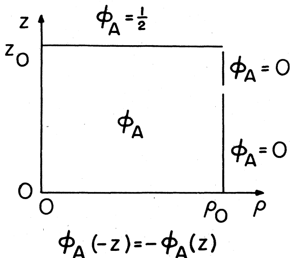
FIG. 54. Boundary condition satisfied by \phi_A in the case of a cylindrical Penning trap. The boundaries are invariant under rotations about the z axis and are antisymmetric under the reflection z \rightarrow -z .
