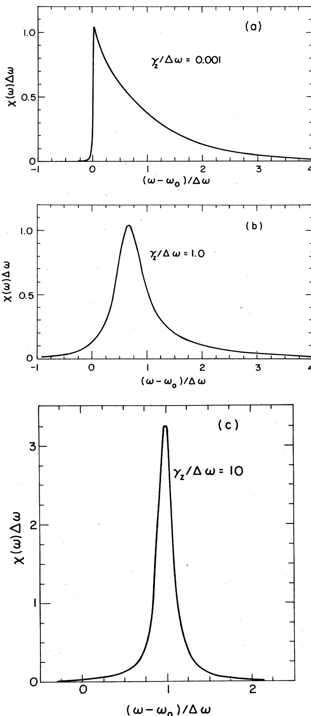
FIG. 26. Line profiles for various values of \gamma_z/\Delta\omega .
