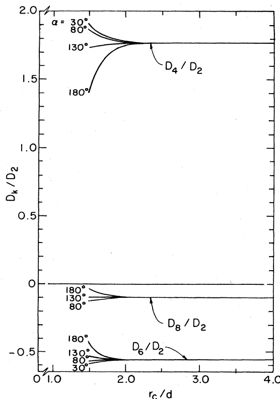
FIG. 47. Ratios of the D_k for asymptotically symmetric Penning traps, with \rho_0 = \sqrt{z_0} . The D_k individually change by nearly 7 orders of magnitude over the range of r_c/d plotted here.
