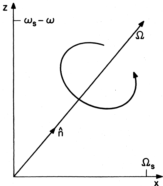
FIG. 22. The axis \hat{n} defined by Eq. (5.10) is stationary in the xz plane of the coordinate system which co-rotates with the drive at the angular frequency \omega . The spin rotates with angular velocity \Omega about this axis.
