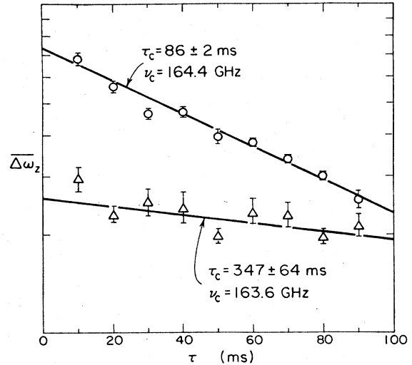
FIG. 41. The energy in the cyclotron motion is proportional to the relativistic mass shift of the axial frequency, as discussed in Sec. VII. In this figure the measured decay with time in such shifts after the cyclotron drive has been turned off are plotted for two values of the cyclotron frequency obtained by changing the magnetic field (Gabrielse and Dehmelt, 1985).
