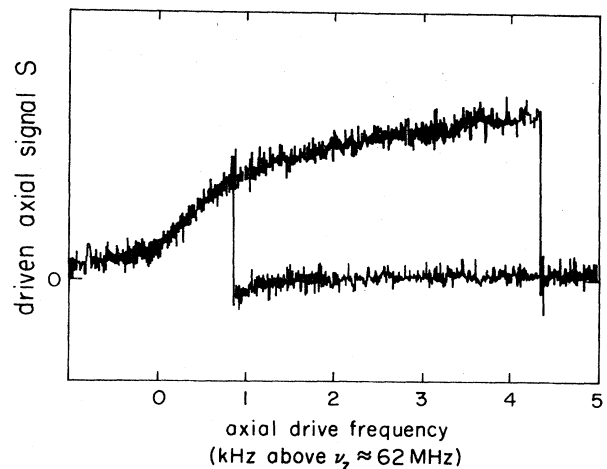
FIG. 13. Anharmonic axial resonance of a single trapped electron in the trap of Fig. 1 observed under detection conditions which correspond to \varphi = 0 in Eq. (3.36). The axial oscillation was made deliberately anharmonic by adjusting the potential applied to the compensation electrodes, and the frequency of the driving force was swept in opposite directions (indicated by the arrows) through resonance. When the trap was tuned to be as harmonic as possible, the axial linewidth was only 6 Hz out of 62 MHz, so that this figure shows the resonant frequency being shifted by approximately 700 linewidths. The shape of these resonances is somewhat different from that of those of Fig. 12 because the detection electronics was saturating due to the large oscillation being observed (Gabrielse and Dehmelt, 1982).
