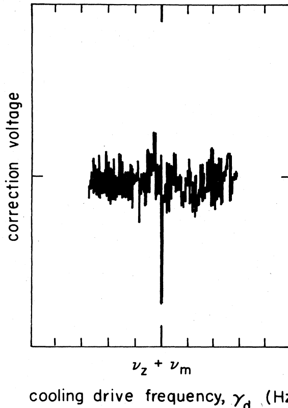
FIG. 18. Narrow feature arising from the decoupling of an axial drive at \nu_z when a cooling drive at \nu_z + \nu_m is applied (Gabrielse and Dehmelt, 1982). Because the axial motion is decoupled from its drive, the shape of this feature depends on the electronics of the locking loop. The width of this feature is at least as narrow as the 0.1-Hz resolution in the drive frequency. Such measurements give a precise determination of the magnetron frequency.
