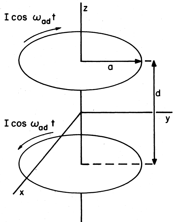
FIG. 23. Effective current loops, which produce the alternating magnetic field near the center of the trap given by Eq. (5.39), with the constant b_1 having the value b_1 = (\pi a^2 I/c) 3d(a^2 + d^2/4)^{-5/2} (in Gaussian units).
