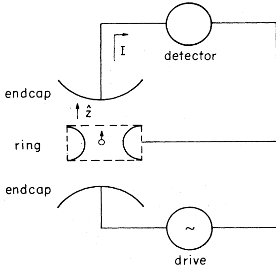
FIG. 4. Sketch indicating the detection and drive of the axial harmonic oscillation.
