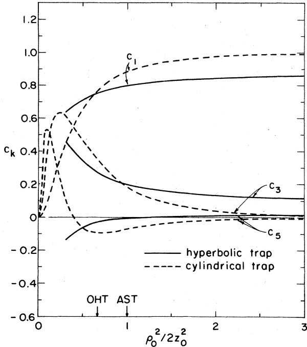
FIG. 53. The coefficients c_k for a hyperbolic Penning trap (with r_c/d=2.5 and \alpha=180^\circ ) and a cylindrical Penning trap. AST and OHT designate asymptotically symmetric and orthogonalized hyperbolic traps, respectively.
