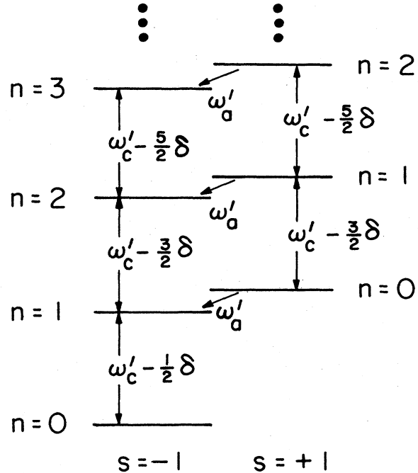
FIG. 34. Relativistic shifts of the spin-cyclotron energy levels for an electron.
