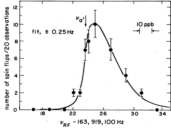
FIG. 28. Experimental anomaly resonance that is not saturated. The solid curve is a fit to the line profile function (6.33) (Van Dyck, Schwinger, and Dehmelt, 1984).
