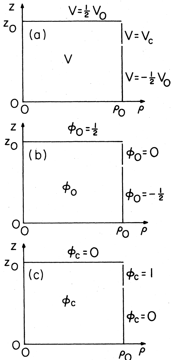
FIG. 56. Boundary conditions for the cylindrical trap in Fig. 55: (a) full potential V ; (b) trapping potential \phi_0 ; (c) compensation potential \phi_c . Invariance under rotations about the z axis and under the reflection z \rightarrow -z is assumed.
