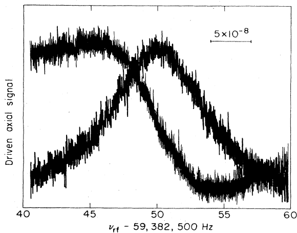
FIG. 10. Two observations of the axial resonance of a single electron. The absorption and dispersion profiles correspond to \varphi=0 and to \varphi=-\pi/2 in Eq. (3.36). Notice that the noise decreases by approximately a factor of 2 on resonance (Van Dyck, Schwinger, and Dehmelt, 1978).
