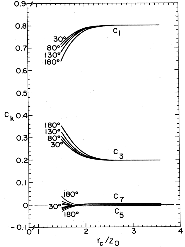
FIG. 52. The coefficients c_k for asymptotically symmetric Penning traps as a function of normalized distance to the compensation electrode for various \alpha .
