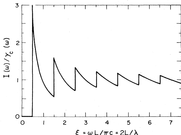
FIG. 36. The decay constant I_P(\omega)/\gamma_c(\omega) for a charged particle moving in the midplane between two perfect conducting planes. The abscissa is in units of \xi , the number of wavelengths at frequency \omega that fit between the planes.
