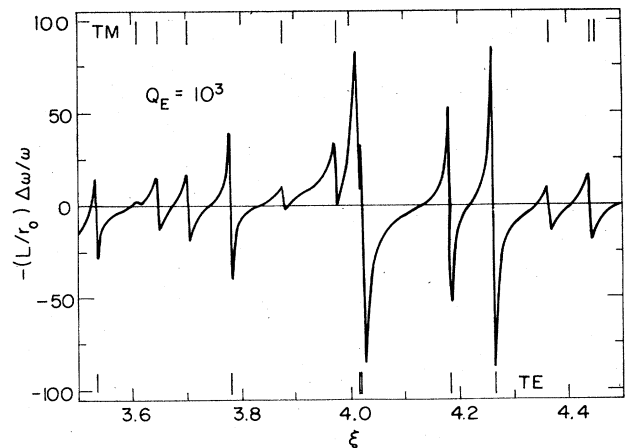
FIG. 42. Frequency shifts corresponding to the decay constants of Fig. 40.
