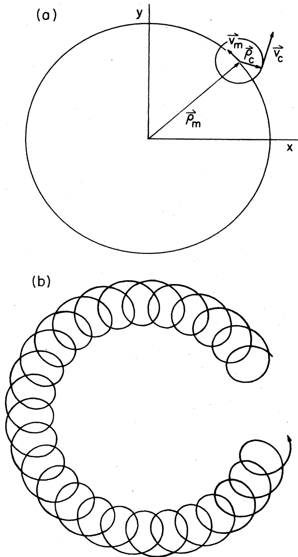
FIG. 7. Projection of the motion of a particle in a Penning trap upon the xy plane. The motion is the superposition of (a) circular magnetron and cyclotron motions producing (b) epicycles. The orbits are not to scale.
