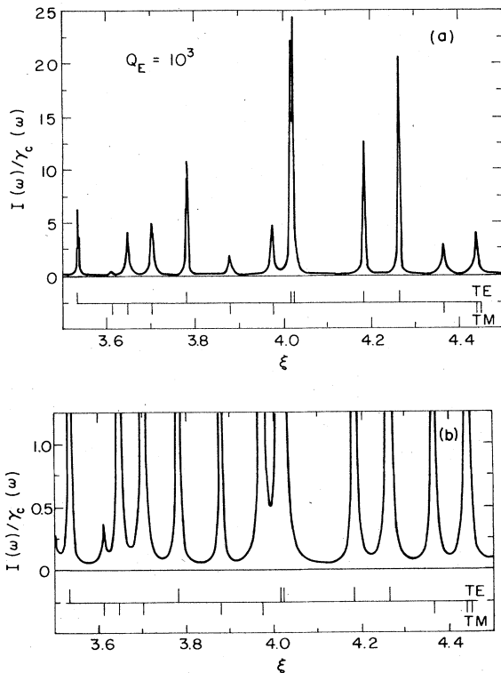
FIG. 40. Cavity effects for R/L=1.186 and Q_E=1000 : (a) decay constant; (b) magnified section of the smaller values of the decay constant.
