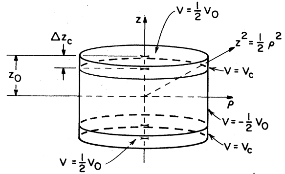
FIG. 55. Electrically compensated cylindrical trap.
