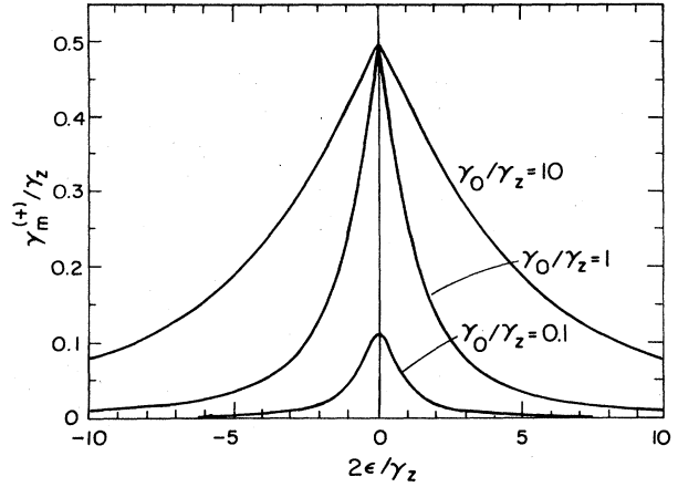
FIG. 19. Line shapes of the cooling rate \gamma_m^{(+)} , as given by Eq. (4.15) for several values of \gamma_0/\gamma_z . With appropriate interpretation, these line shapes apply to the analogous decay constants of Sec. III.C as well.
