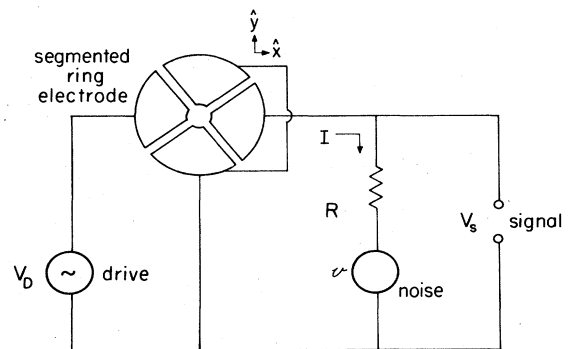
FIG. 15. Idealized radio-frequency circuit, which could be used to damp and detect the cyclotron oscillation of a trapped particle when this frequency is a radio frequency. The x component of the cyclotron motion induces a current I through the resistor. The cyclotron motion is driven by the oscillatory potential V_D and by the Johnson noise from the resistor v , while the signal voltage V_S is detected. This circuit is directly analogous to the circuit in Fig. 9 for the axial motion.
