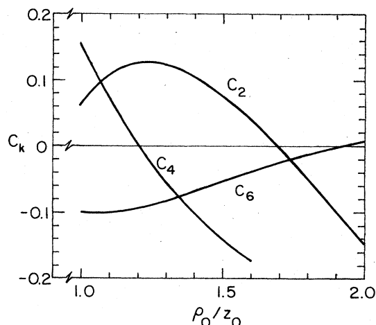
FIG. 57. Lowest-order C_k for a cylindrical trap in the limit of a vanishing compensation electrode, \Delta z_c \rightarrow 0 .
