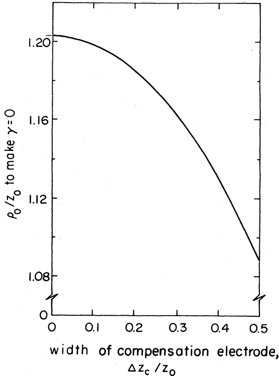
FIG. 58. The ratio \rho_0/z_0 required to make \gamma=0 , for a cylindrical Penning trap, as a function of the width of the compensation electrode.
