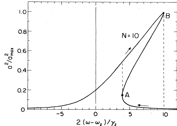
FIG. 12. The resonance profiles that would be observed experimentally by sweeping the frequency of the driving force up or down through the anharmonic axial resonance given for N = 10 in Fig. 11.
