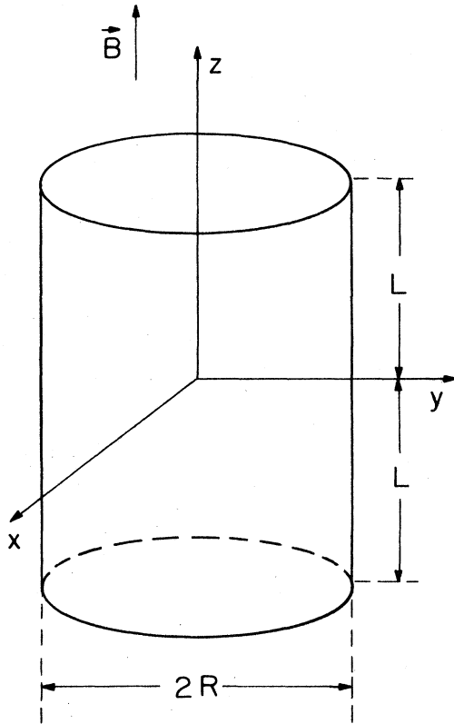
FIG. 35. Cylindrical cavity of radius R and length 2L . A uniform magnetic field \mathbf{B} is aligned along the axial symmetry axis of the cavity, and the charged particle is in a small orbit in the center of the cavity.
