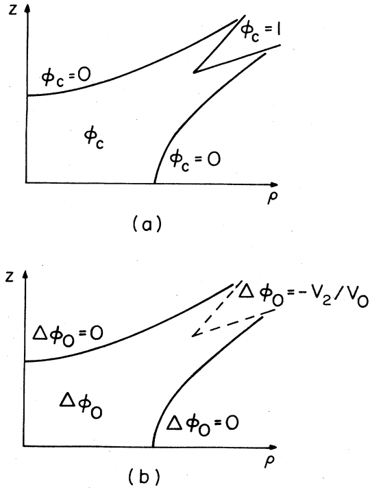
FIG. 44. Boundary conditions that uniquely determine the solutions to Laplace's equation, \phi_c in (a) and \Delta\phi_0 in (b). The boundaries are invariant under rotations about the z axis and under the reflection z \rightarrow -z . The dashed boundary in (b), located at the compensation electrode, is not an equipotential. The potential at each point on this boundary is given by the value of -V_2/V_0 at this point.
