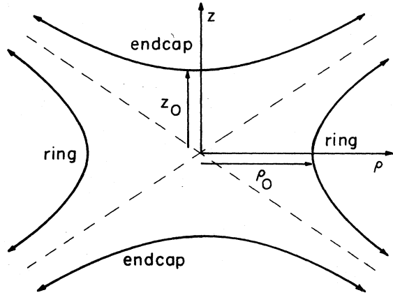
FIG. 6. Axially symmetric electrodes are used to produce a quadrupole potential of the form given by Eq. (2.2). The dashed lines represent the cones that are the asymptotes of the hyperbolas of revolution.
