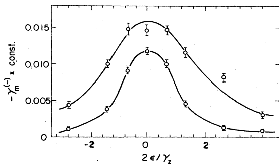
FIG. 21. Experimental observations of the heating line shapes \gamma_m^{(-)}(\epsilon) by Gabrielse and Dehmelt (1982), as described in the text. The error bars are statistical, and smooth curves are included to aid the eye. The vertical scale is the inverse of the time required to heat the magnetron motion from the smallest obtainable magnetron radius to the larger, observable radius. Such measurements are rather time consuming, taking about 3 h of averaging time for each of the points farthest from the center. The upper, broader curve corresponds to a higher power, so that power broadening is clearly demonstrated, but the power ratio is not well calibrated, owing to the very small amplitude of the drives and the presence of radio-frequency leakage paths. Moreover, it is difficult for the existing electronics to follow the fast increase in the magnetron radius near resonance, making the heights of the center points somewhat suspect.
