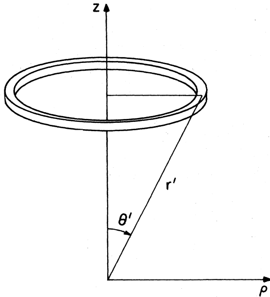
FIG. 24. Coordinates for a little ring of magnetization.
