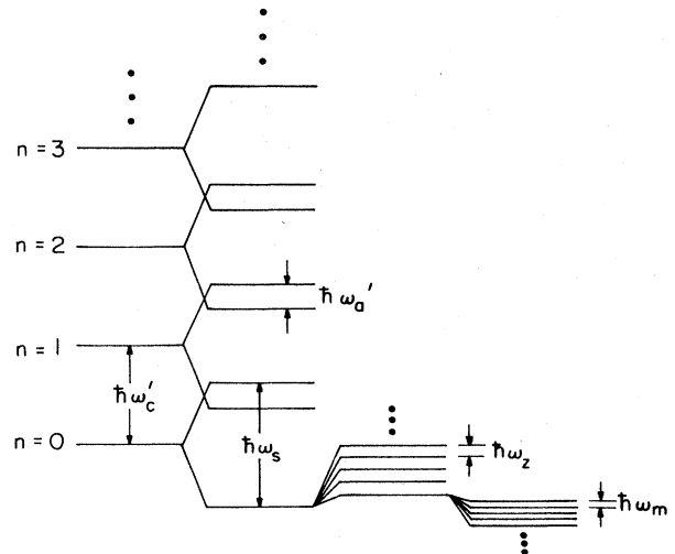
FIG. 8. Splitting of geonium energy levels for an electron (not to scale). The ladder on the far left represents the basic cyclotron energy levels. Progressing to the right, these levels are split first by the spin ( = \frac{1}{2} ), then by the axial binding, and finally by the magnetron motion. The magnetron levels are inverted, since the motion is unbound.
