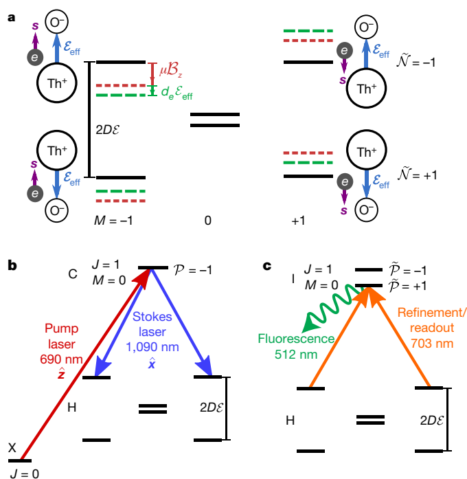
Fig. 1 | Energy levels of thorium monoxide and laser transitions. The addressed transitions are shown for one of several possible experimental states. a , Levels of the state H, J=1 in external electric ( \mathcal{E} ) and magnetic ( \mathcal{B} ) fields. The orientation of the effective electric field, \mathcal{E}_{\text{eff}} , is shown by blue arrows and that of the spin of the electron, s , by purple arrows. The energy shifts \mu\mathcal{B}_z (brown) and d_e\mathcal{E}_{\text{eff}} (green) due to the magnetic moment \mu and the EDM d_e , respectively, are shown. The \tilde{N} = \pm 1 states are split by 2D\mathcal{E} \approx 200 MHz owing to the Stark effect, where D is the H-state electric dipole moment. b , STIRAP efficiently transfers population from the ground state |X, J=0\rangle to a spin-aligned superposition of one molecule orientation, \tilde{N} = +1 or \tilde{N} = -1 ( \tilde{N} = -1 shown here). STIRAP uses two lasers, the pump laser (red arrow; X–C, 690 nm, polarized along \hat{z} ) and the Stokes laser (blue arrows; C–H, 1,090 nm, polarized along \hat{x} ). c , The refinement laser (orange) removes imperfections in the spin-aligned state prepared by STIRAP. The readout laser (orange) excites the molecule from its original orientation, \tilde{N} = +1 or \tilde{N} = -1 ( \tilde{N} = -1 shown here), to an isolated J=1, M=0 level in state I. This state can have either parity, \tilde{P} = +1 or \tilde{P} = -1 ( \tilde{P} = +1 shown here). The I state decays via spontaneous photon emission, and we detect the resulting fluorescence (green wavy arrow).
