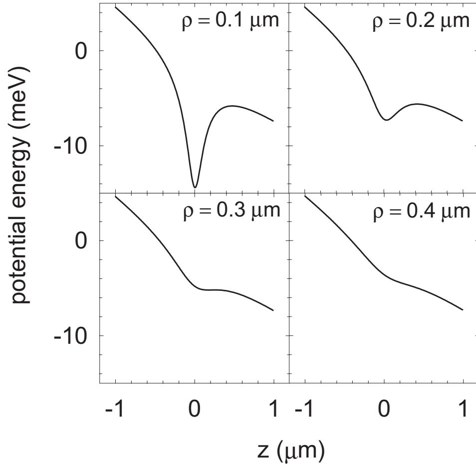
Figure 6.9: In an applied electric field the axial well depth decreases and moves towards positive z as the positron - antiproton radial separation increases. All plots are for an applied field of 60 \text{ Vcm}^{-1} .
