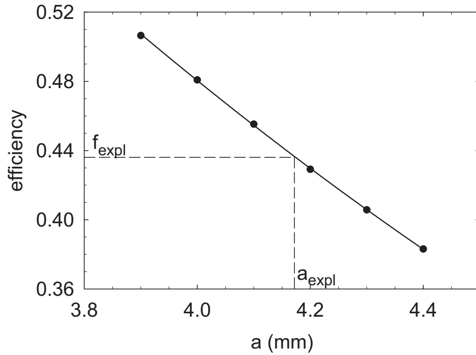
Figure 4.10: Numerical calculation of the transfer efficiency for a cloud of 1.4 million positrons with a given radius. Each point on the graph represents a numerical calculation of the transfer efficiency through the ball valve.
