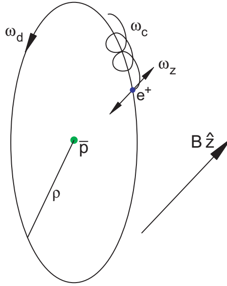
Figure 6.8: In a circular guiding center atom the positron oscillates axially in the Coulomb field of the antiproton, and the guided center of the cyclotron orbit drifts around the antiproton at a radius \rho .
