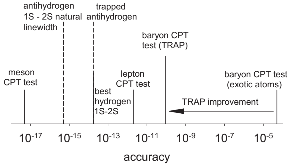
Figure 1.1: Antihydrogen spectroscopy to the level now attained in hydrogen is highly competitive with the most accurate CPT tests in the baryon, lepton and meson systems.
