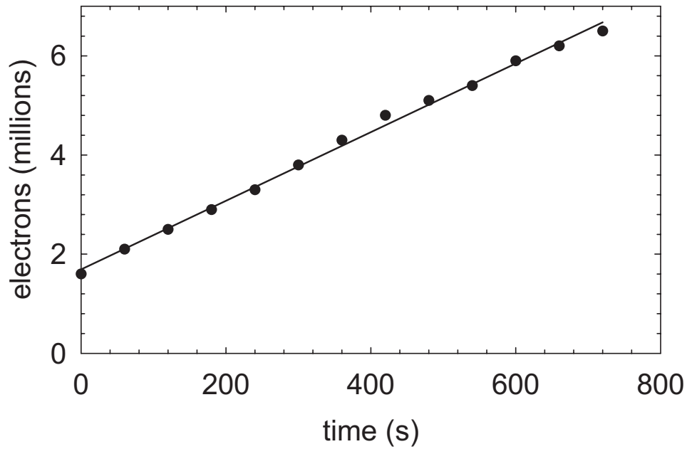
Figure 3.3: Electron loading directly onto Etrap from the radioactive source.
